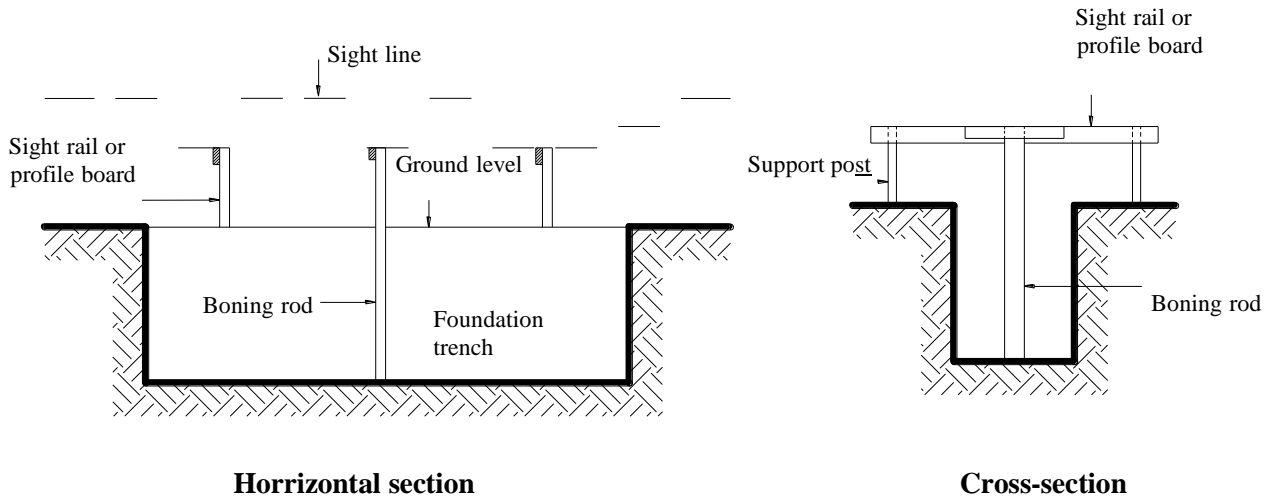
Fig 2.2c Boning rod
