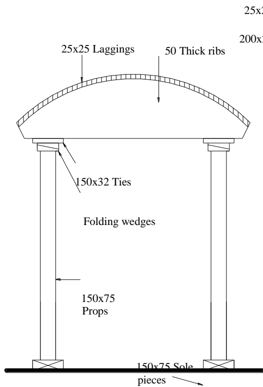
Fig 2.9b Center for small span arches
