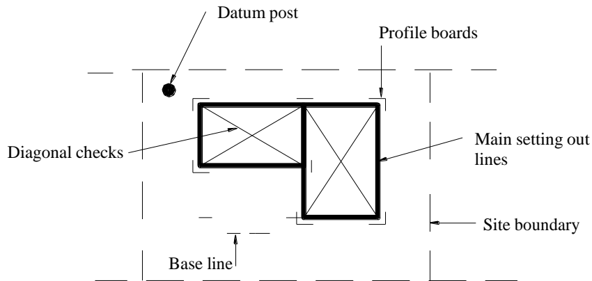
Fig 2.2a Setting out
