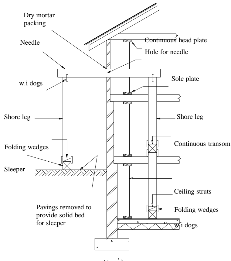
Fig 2.6a Dead shoring
