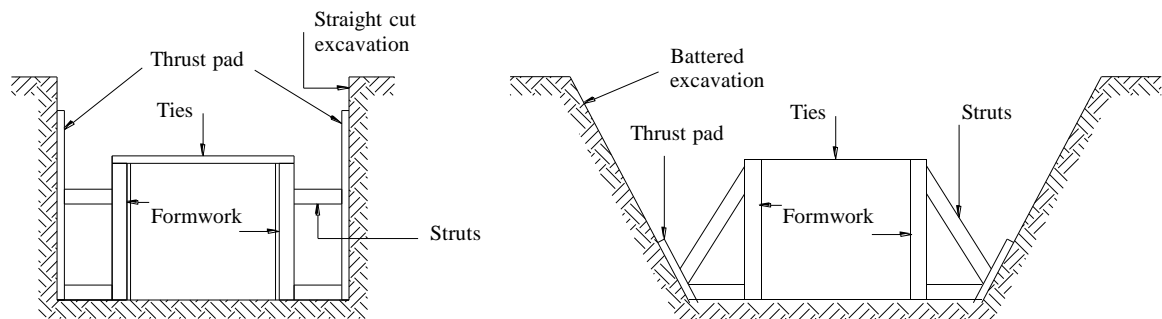
Fig 2.9a Foundation formwork
