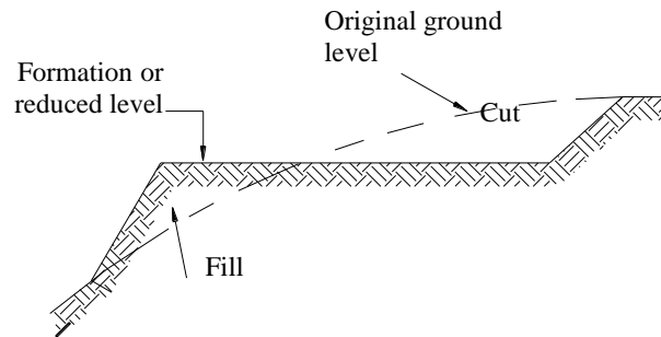
Fig 2.1a Cut and fill method of leveling
