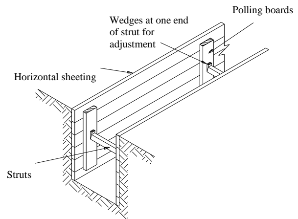
Fig 2.3d Timbering in dry loose soils
