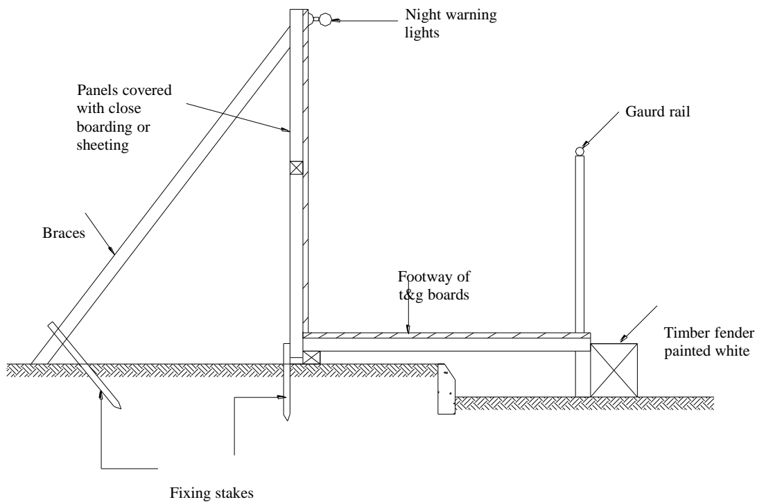
Fig 2.5a Free standing vertical hoarding
