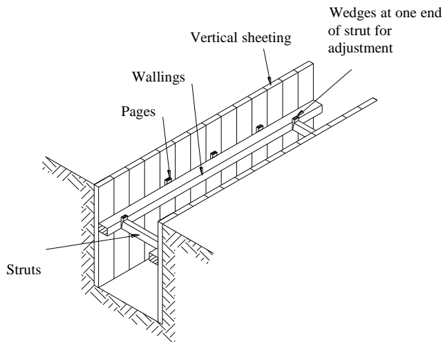
Fig 2.3a Timbering in hard soils
