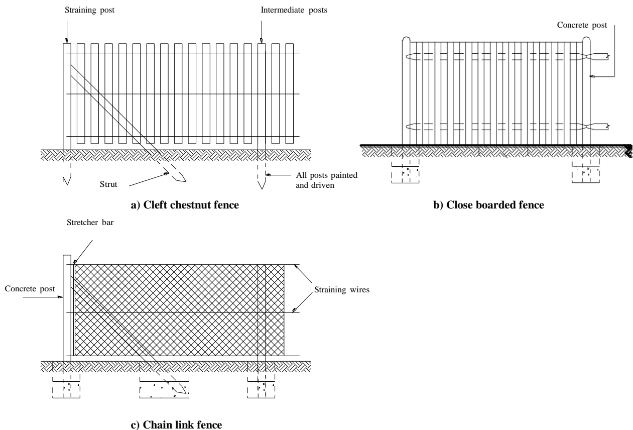
Fig 2.4a Types of site fencing
