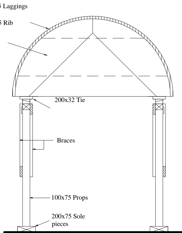
Fig 2.9c Framed center for medium span arches (up to 1500mm)
