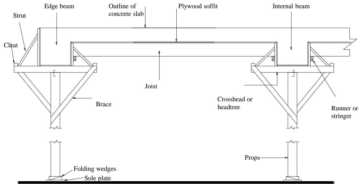
Fig 2.9d Slab formwork
