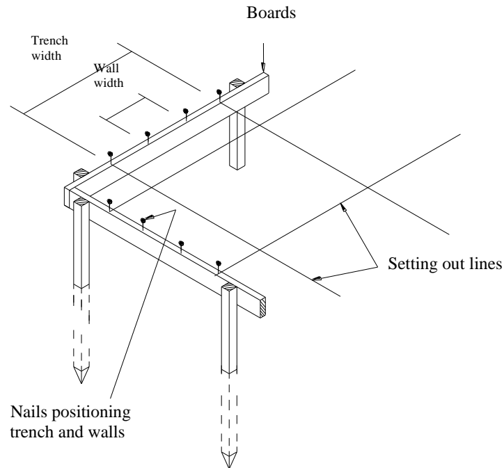
Fig 2.2b Profile board
