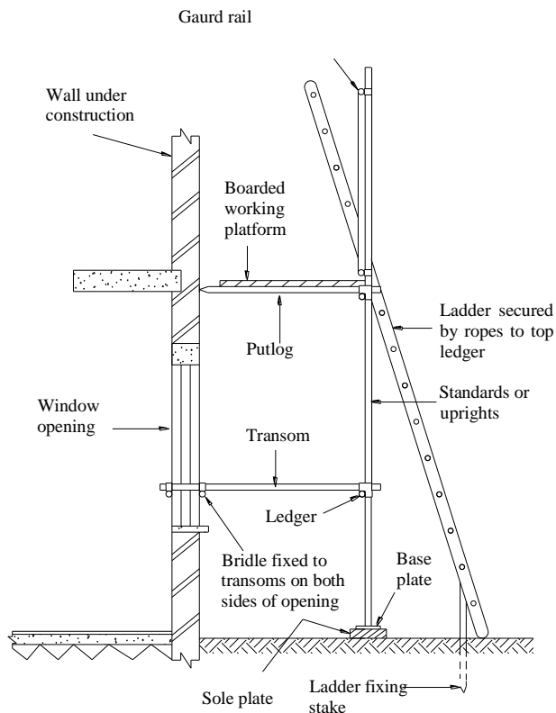
Fig 2.7a Putlog scaffolding
