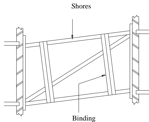
Fig 2.6c Flying shore
