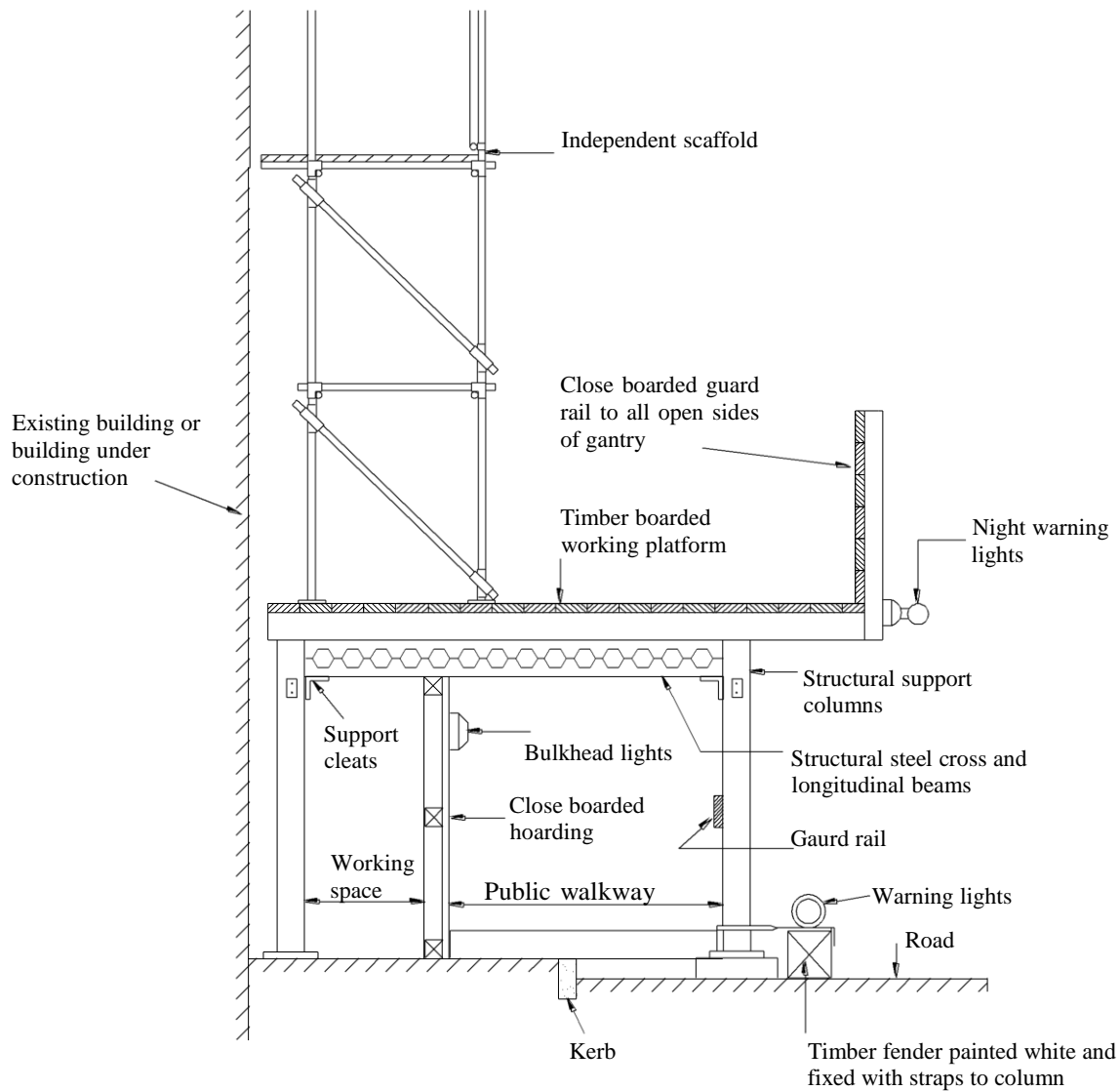
Fig 2.8a Gantry
