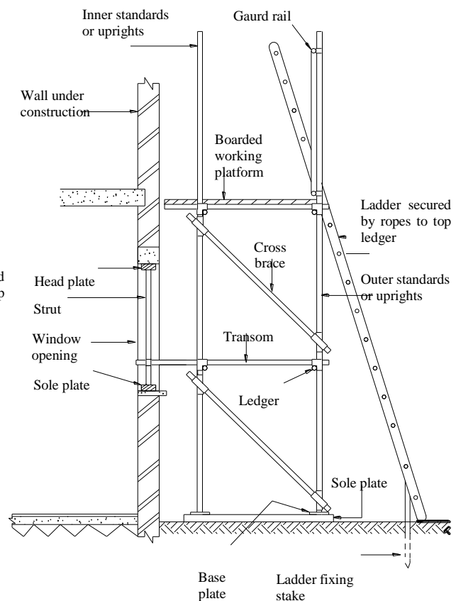
Fig 2.7b Independent scaffolding
