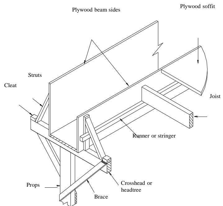
Fig 2.9c Beam formwork
